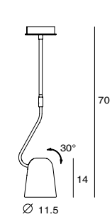
Dobi Pendant Tube 70 SQ-2181PR-70 E14 Max 25W/ 6W LED Shade rotatable NW : 1.1kg
