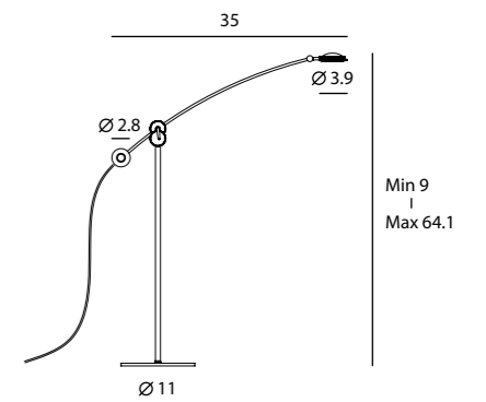
Planet Floor SLD-100FRTE LED 1 x 8.6W (3000K, Ra>90, 600lm) multi-direction adjustable Touch dimmer, adaptor driver Materials : steel, copper (gear) Color : copper
