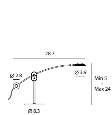
Planet Table SLD-100DRTE LED 1 x 8.6W (3000K, Ra>90, 600lm) multi-direction adjustable Touch dimmer, adaptor driver Materials : steel, copper (gear) Color : copper
