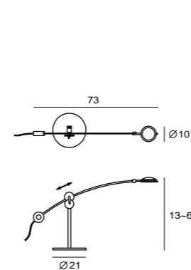
PLANET D SLD-100DRTE LED 8.6W 3000K 600lm CRI90 steel, copper copper 紅銅 multi-direction adjusted touch dimmer
