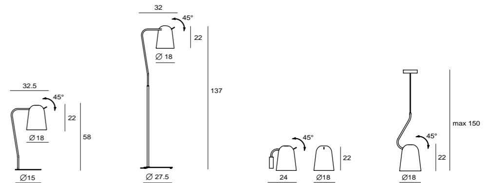
DODO D SQ-218DR E27 1 x Max 12W CFL shiny white/ matt black/ copper 亮白/ 霧黑/ 紅銅 adjustable lampshade
