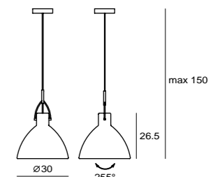
LAITO P L SQ-897MP E27 1 x Max 23W CFL matt black/chrome/ copper 霧黑/ 鉻/ 紅銅 shade rotatable
