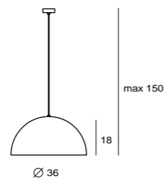
DOME P M SQ-360MP E27 1 x Max 12W CFL matt black/ shiny white/ copper 霧黑/ 亮白/ 紅銅 swirling reflector, bulb cover
