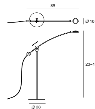
PLANET F SLD-100FRTE LED 8.6W 3000K 600lm CRI90 steel, copper copper 紅銅 multi-direction adjusted touch dimmer
