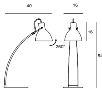
LAITO WOOD D SQ-893DWR E27 1 x Max 12W CFL beech, steel matt pure white/ matt black 霧白/ 霧黑 shade rotatable
