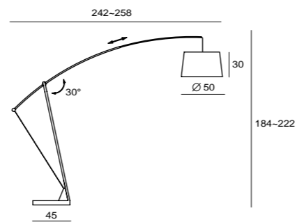
ARCHER F XL SQ-603FLR E27 3 x Max 23W CFL fabric, steel, beech adjustable arm
