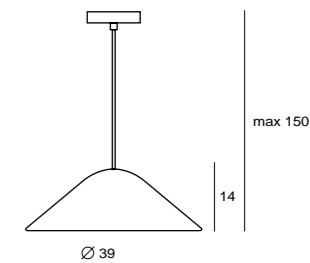
DAMO P SQ-339MP E27 2 x Max 12W CFL matt black/ copper 霧黑/ 紅銅
