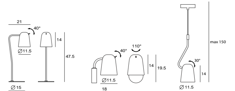
DOBI D SQ-2181DR E14 1 x Max 25W adjustable lampshade shiny white + matt brass/ copper + matt black 亮白+霧金/紅銅+霧黑
