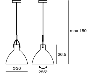
LAITO P L SQ-897MP E27 1 x Max 77W Halogen matt black/ matt pure white/ chrome/ copper shade rotatable Canopy: A Plate: A
