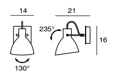
LAITO W SQ-893MWR E27 1 x Max 46W Halogen matt black/ matt pure white/ chrome/ copper shade rotatable Canopy: B2 Plate: A5
