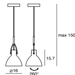
LAITO P M SQ-8961MP E27 1 x Max 46W Halogen matt black/ matt pure white/ chrome/ copper shade rotatable Canopy: A Plate: A
